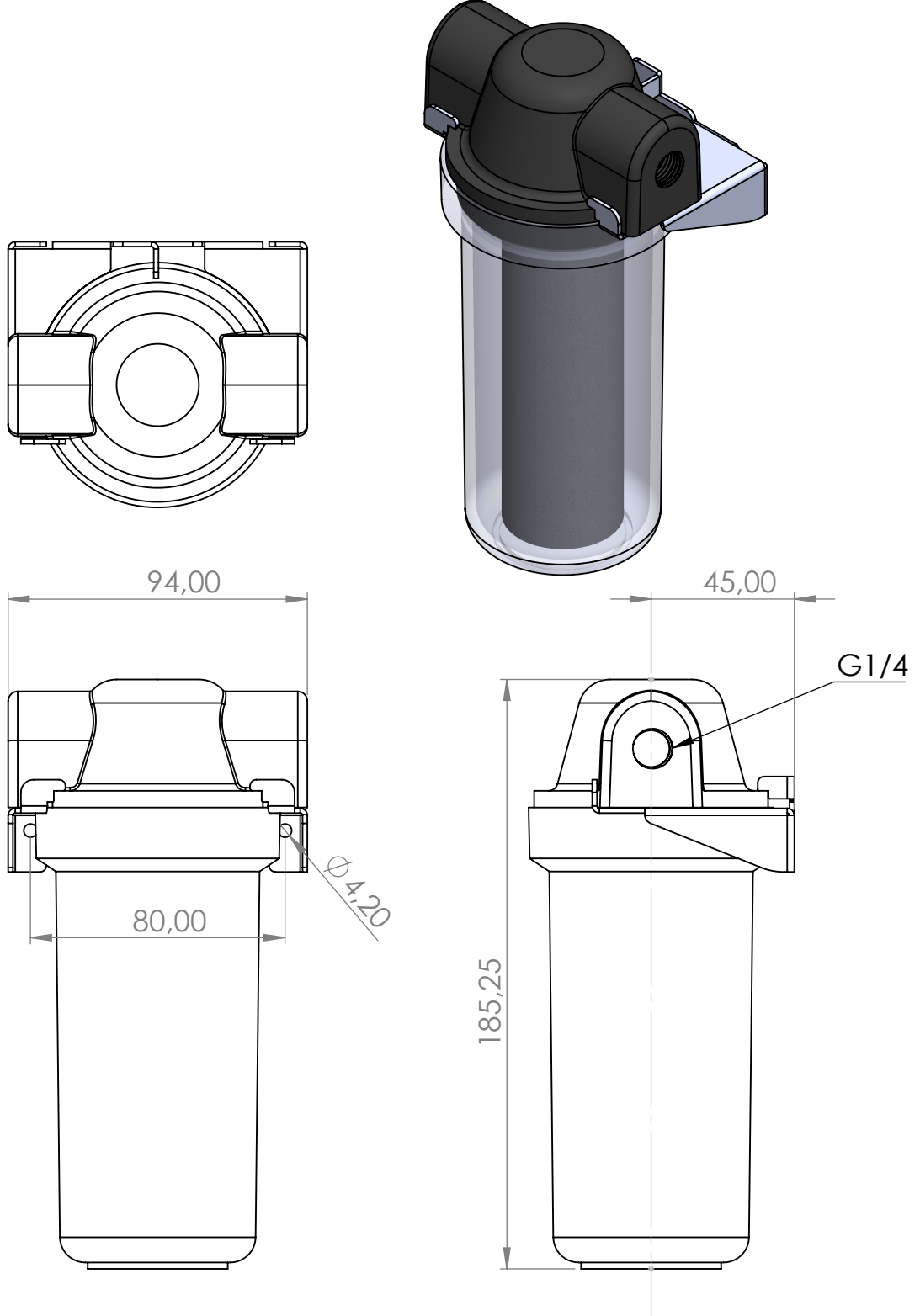
FILTER SET FB10 -18cm 1/4" Filter Housing -Stainles Filter -Stainles Mantage Part
